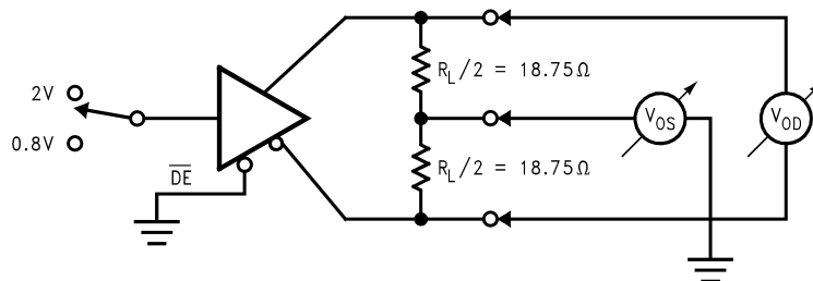
Figure 5. Differential Driver DC Test
