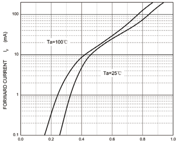
Forward Characteristics
