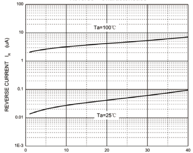
Reverse Characteristics
