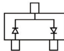
Equivalent Circuit
