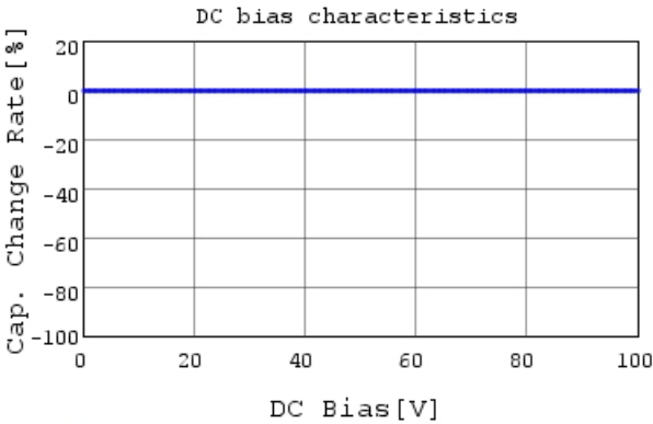
GJM0335G2A4R7WB01 C-DC bias capchange, 25.0C
