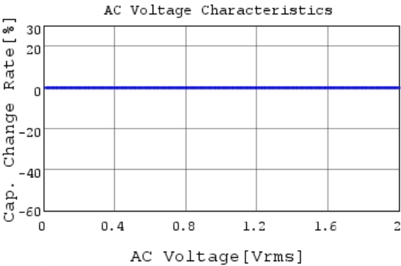
GJM0335G2A4R7WB01 C-AC Voltage capchange, Dc
