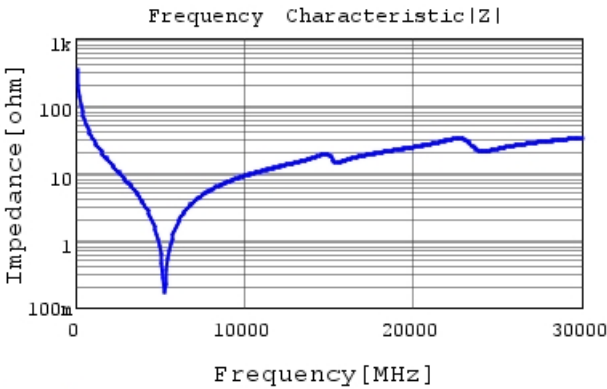
GJM0335G2A4R7WB01 |Z| DCOV, 25degC
