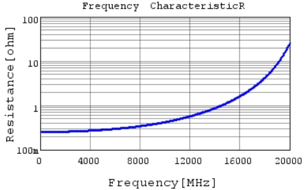
GJM1555C1HR90WB01 R DCOV, 25degC
