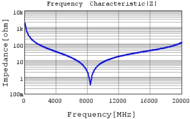
GJM1555C1HR90WB01 |Z| DCOV, 25degC
