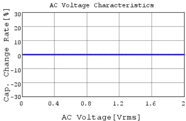
GJM1555C1HR90WB01 C-AC Voltage capchange, Dc
