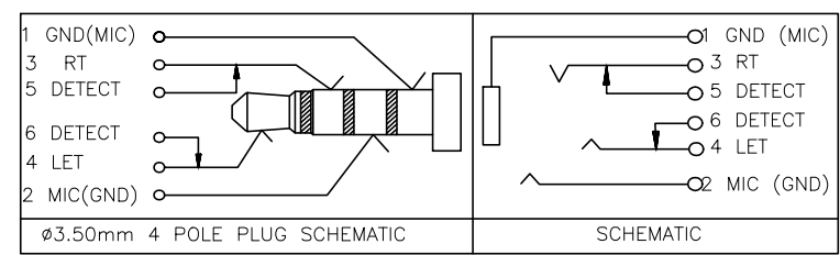
ø3.50mm 4 POLE PLUG DETAIL DRAWING
