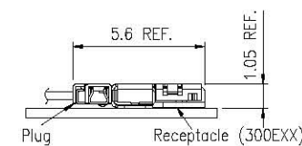
Mating condition
