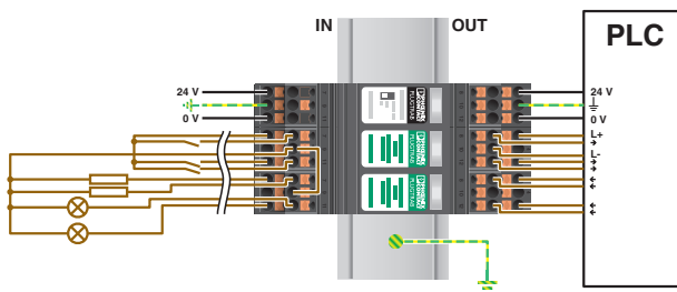
Application drawing
