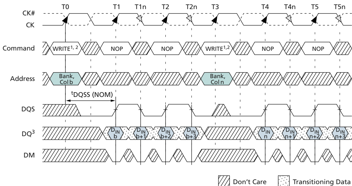
Figure 42: Nonconsecutive WRITE-to-WRITE
