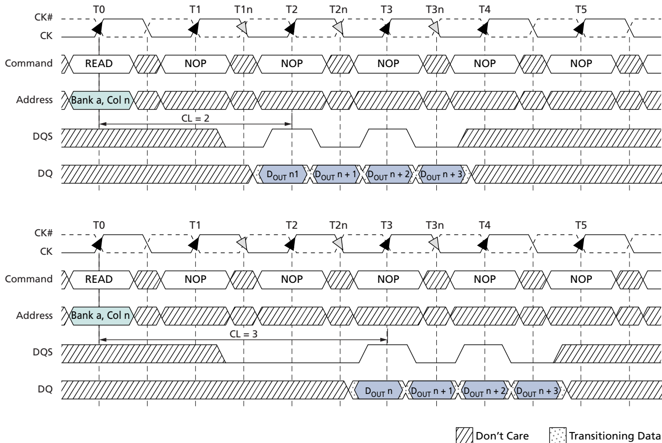
Figure 28: READ Burst
