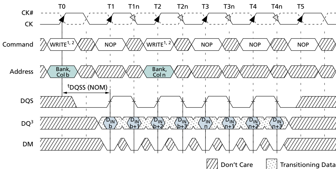
Figure 41: Consecutive WRITE-to-WRITE
