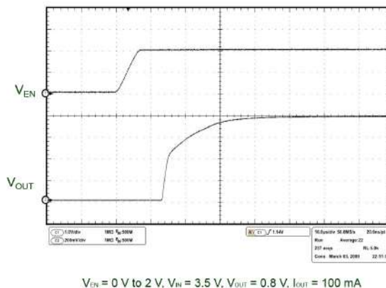
Figure 29. Enable transient
