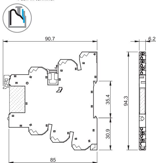
Types 39.60/39.60.3 39.61/39.61.3 Push-in terminal
