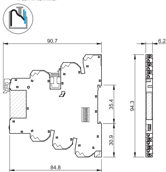
Types 39.90 39.91 Push-in terminal
