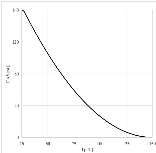
Figure 15: Avalanche Energy
