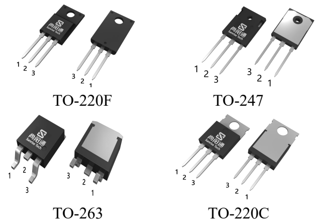
Figure 2 Package Types of SRC60R078BS
