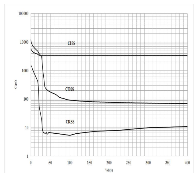
Figure 16: Typ. Capacitances
