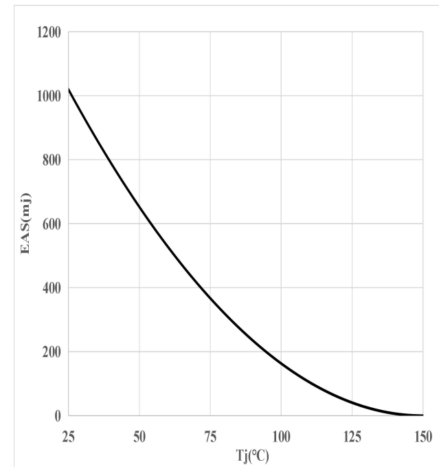
Figure 15: Avalanche Energy
