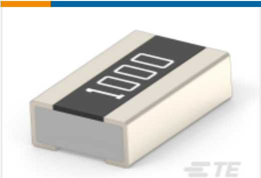
TE Part #2-2176554-4 3430 A2 1% 8R2 150ppm 1k RL
