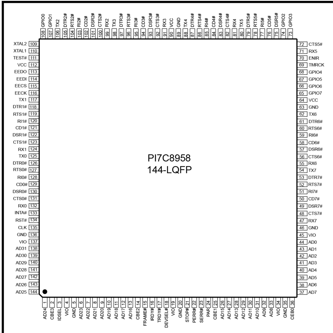
Figure 3-2 Pin Out
