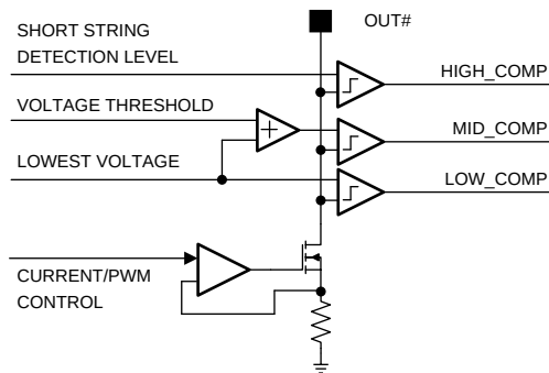
Figure 11. Comparators for Adaptive Voltage Control and LED Fault Detection
