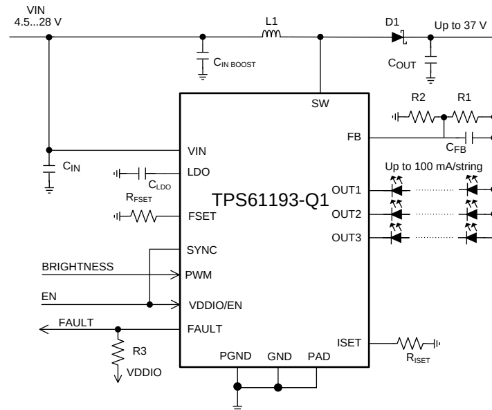
Figure 20. Three Strings 100 mA/String Configuration
