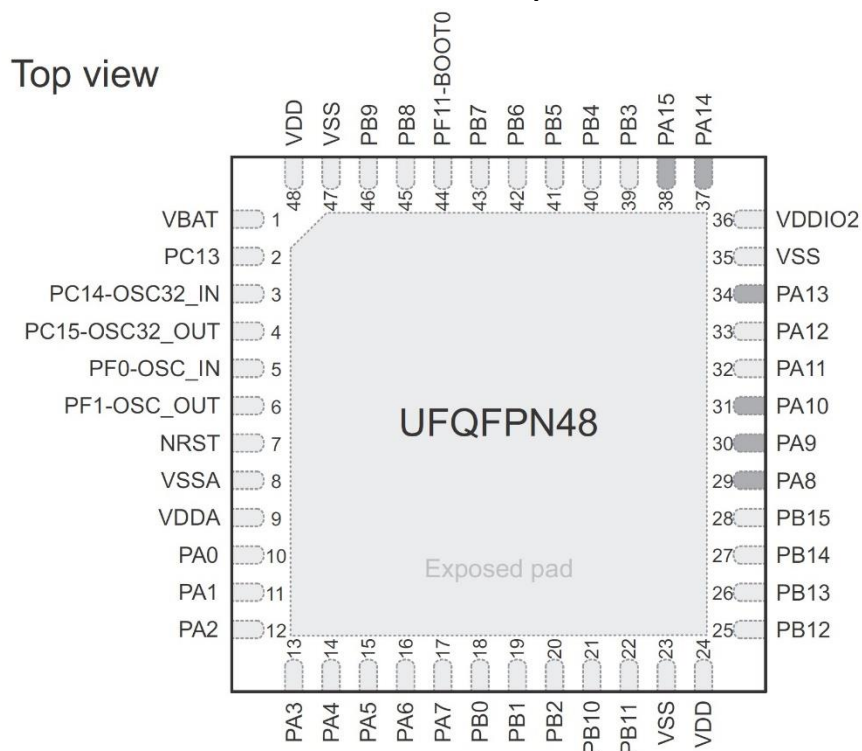
FCM32x042x UFQFPN48 pinout
