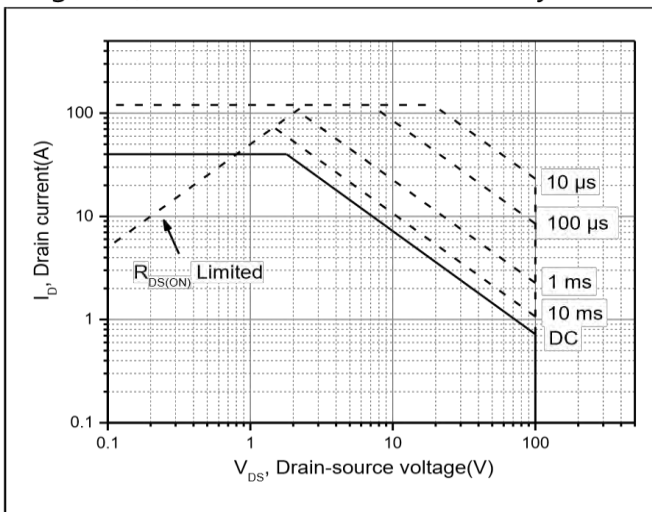
Figure 9, Safe operation area T_C = 25^\circ C
