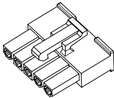
POSITIVE LATCH SCALE 2:1
