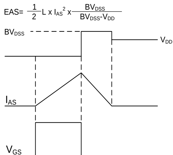
Fig.8 EAS Waveform
