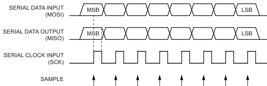
Figure 3-94. Serial Programming Waveforms
