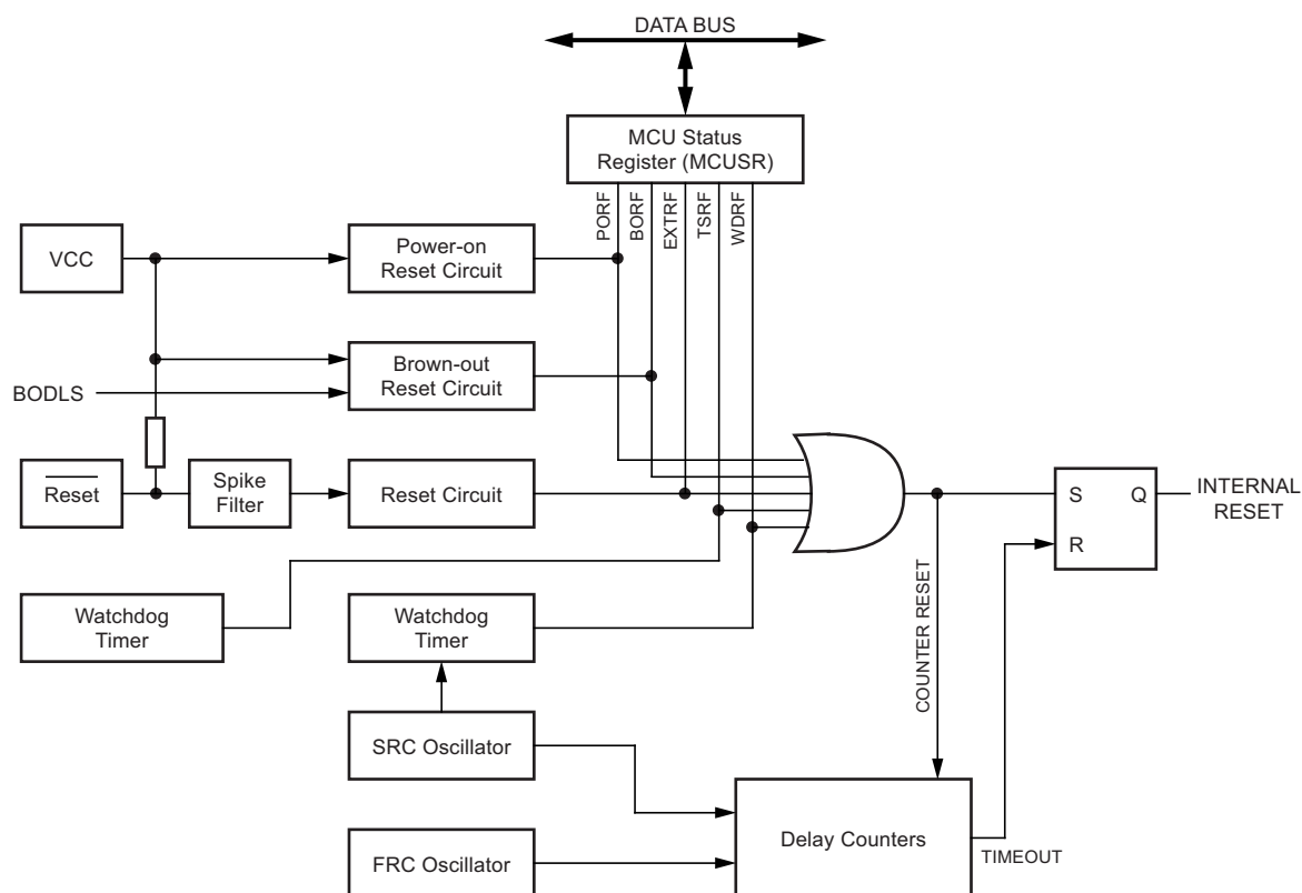
Figure 3-15. Reset Logic
