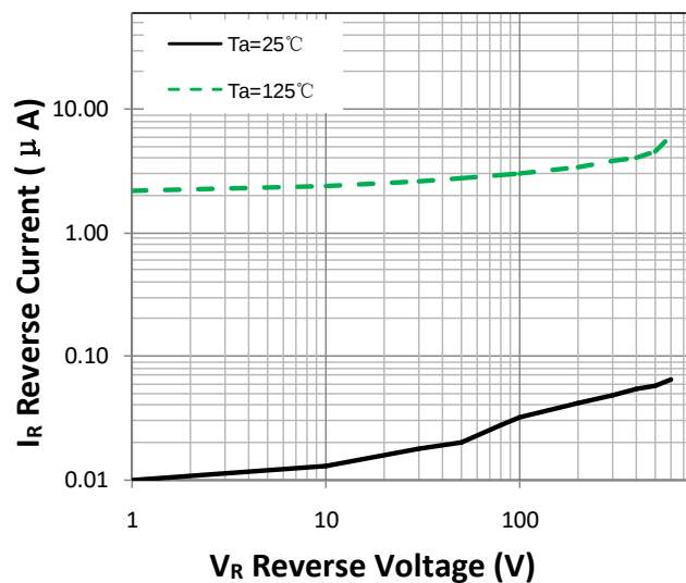
Figure 2. Reverse Characteristic (typ.)
