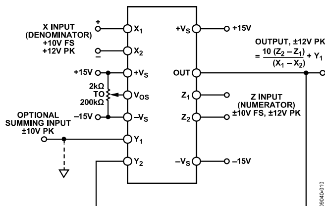
Figure 9. Basic Divider Connection
