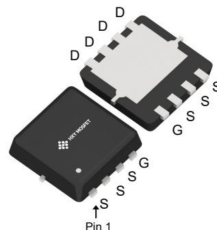
DFN3X3-8L (WDFN-8(3.3x3.3))
