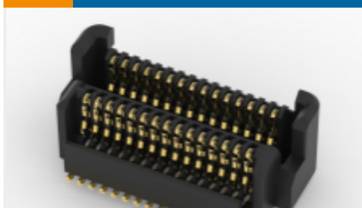
TE Part #2291283-2 0.5MM FPH BTB, 4H/30POS/15U/TR/WOB/B
