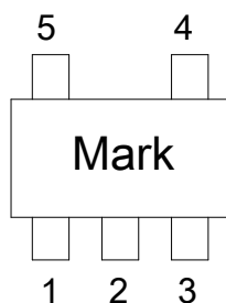
SOT-23-5L(Top View)
