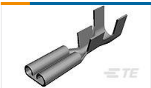
TE Part #140719-2 110 FASTON,REC.,22-18 AWG,TPBR
