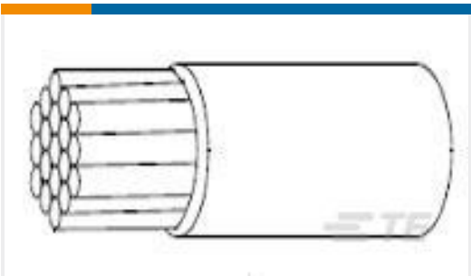
TE Part #216113-001 22759/32-20-9
