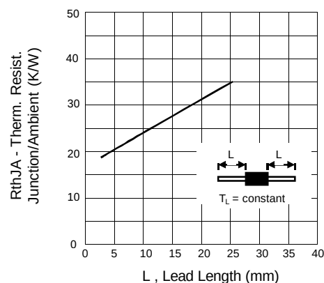
FIG.3 - MAXIMUM THERMAL RESISTANCE vs. LEAD LENGTH
