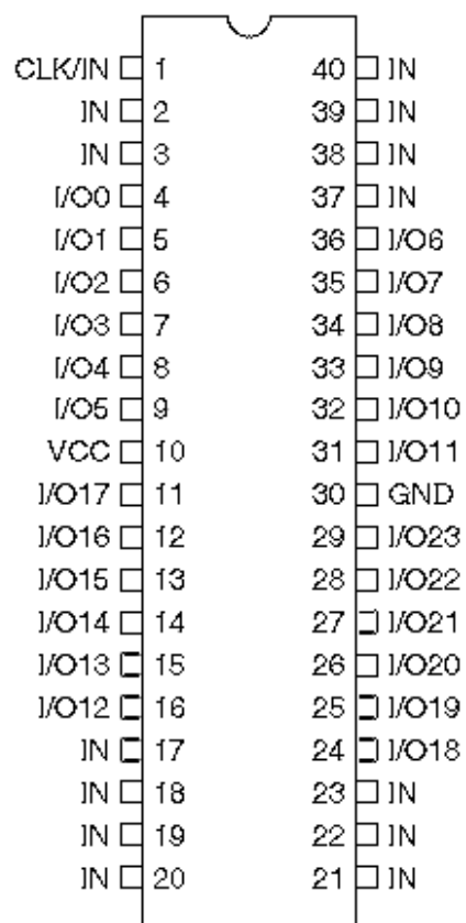
CERDIP
