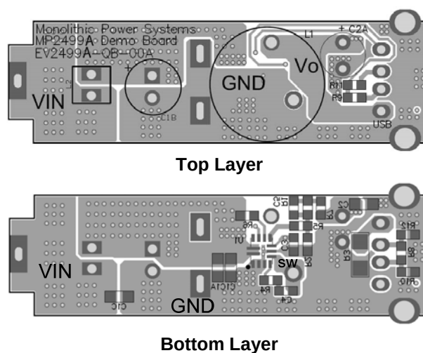
Figure 9: Recommended Layout
