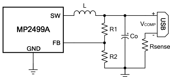
Figure 3: Output Line Drop Compensation
