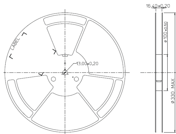
Figure 14 Reel Dimension
