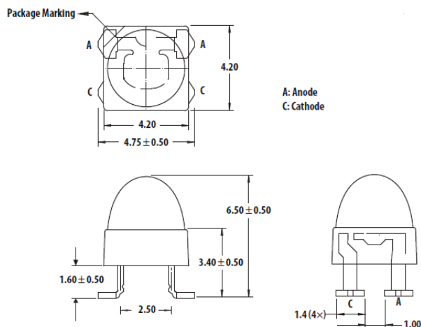
Figure 1 Package Dimensions
