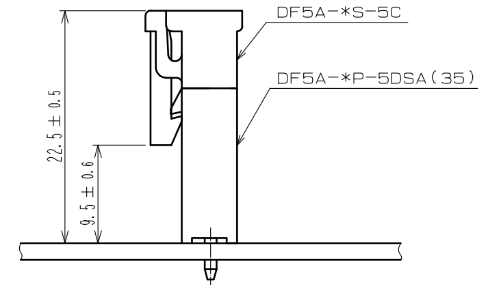
APPLICATION DIAGRAM
