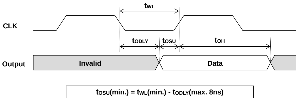
Figure 2 Output timing
