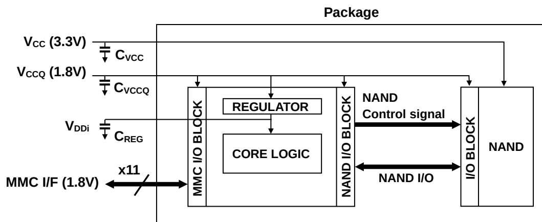
Figure 1 THGAMRT0T43BAIR Block Diagram
