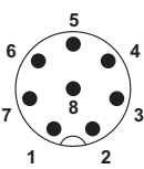
Pin assignment M12 plug, 8-pos., view plug side
