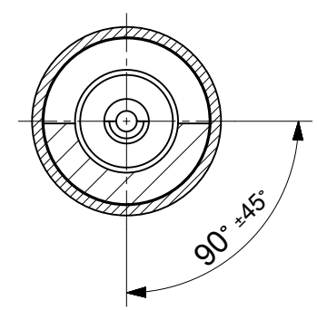
Solderpot position
