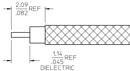
RECOMMENDED STRIP DIMENSIONS FOR NON JACKETED CABLES SR .047
