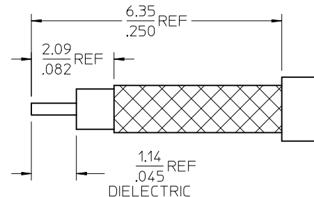
RECOMMENDED STRIP DIMENSIONS FOR JACKETED CABLES
