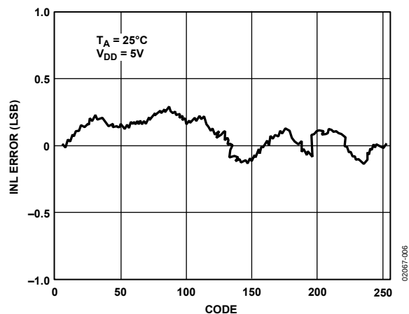
Figure 6. AD5307 INL
