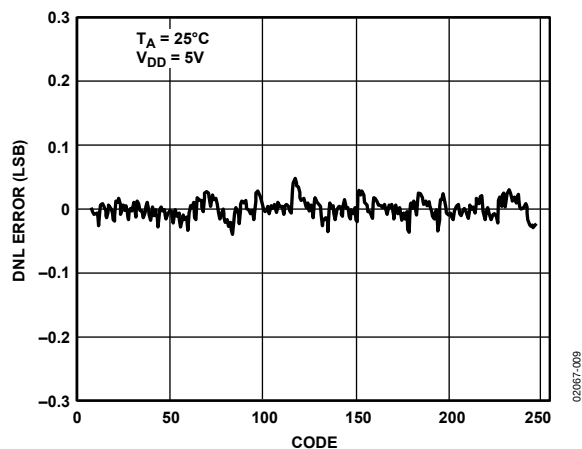
Figure 9. AD5307 DNL
