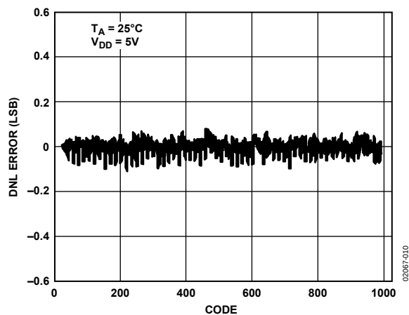
Figure 10. AD5317 DNL
