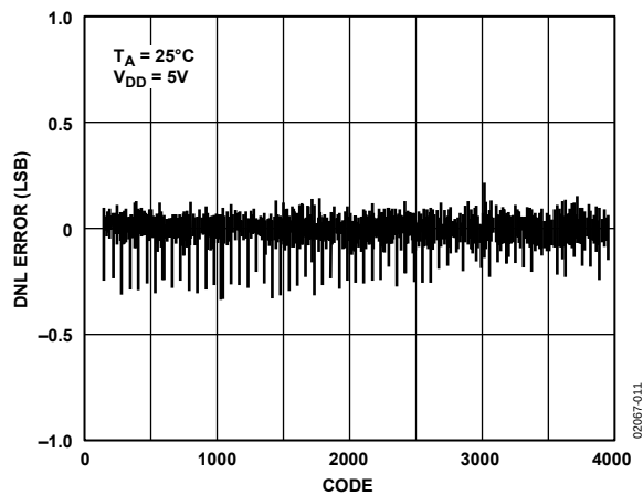
Figure 11. AD5327 DNL
