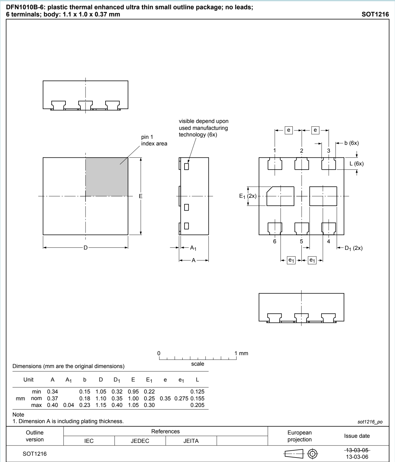
Fig. 19. Package outline DFN1010B-6 (SOT1216)
