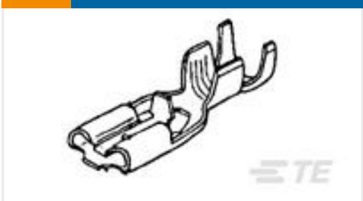
TE Part #170326-5 187 PL MKII REC. 18-14AWG PTPB
