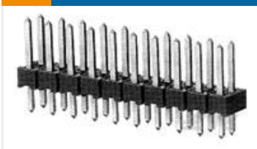
TE Part #5-146254-3 06 MODII HDR DRST B/A .100CL
