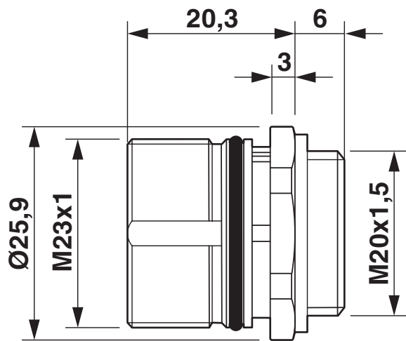
Dimensional drawing
