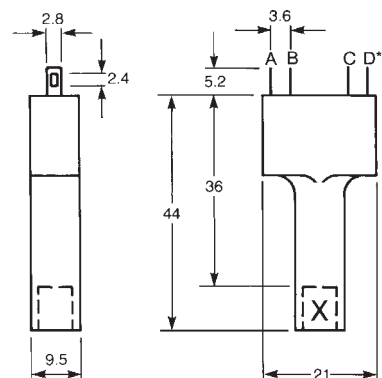
Terminal Arrangement
