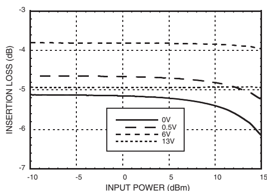
Insertion Loss vs. Pin @ 4 GHz
