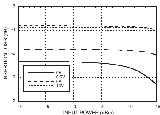
Insertion Loss vs. Pin @ 8 GHz
