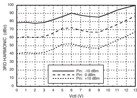
Third Harmonics vs. Vctl, F = 6 GHz
