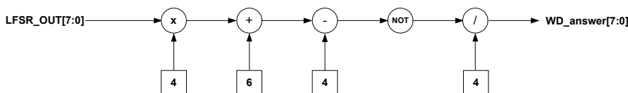
Figure 12. Watchdog Answer Calculation
