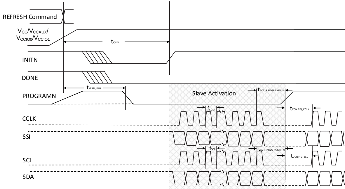
Figure 3.15. Slave SPI/I²C/I³C POR/REFRESH Timing
