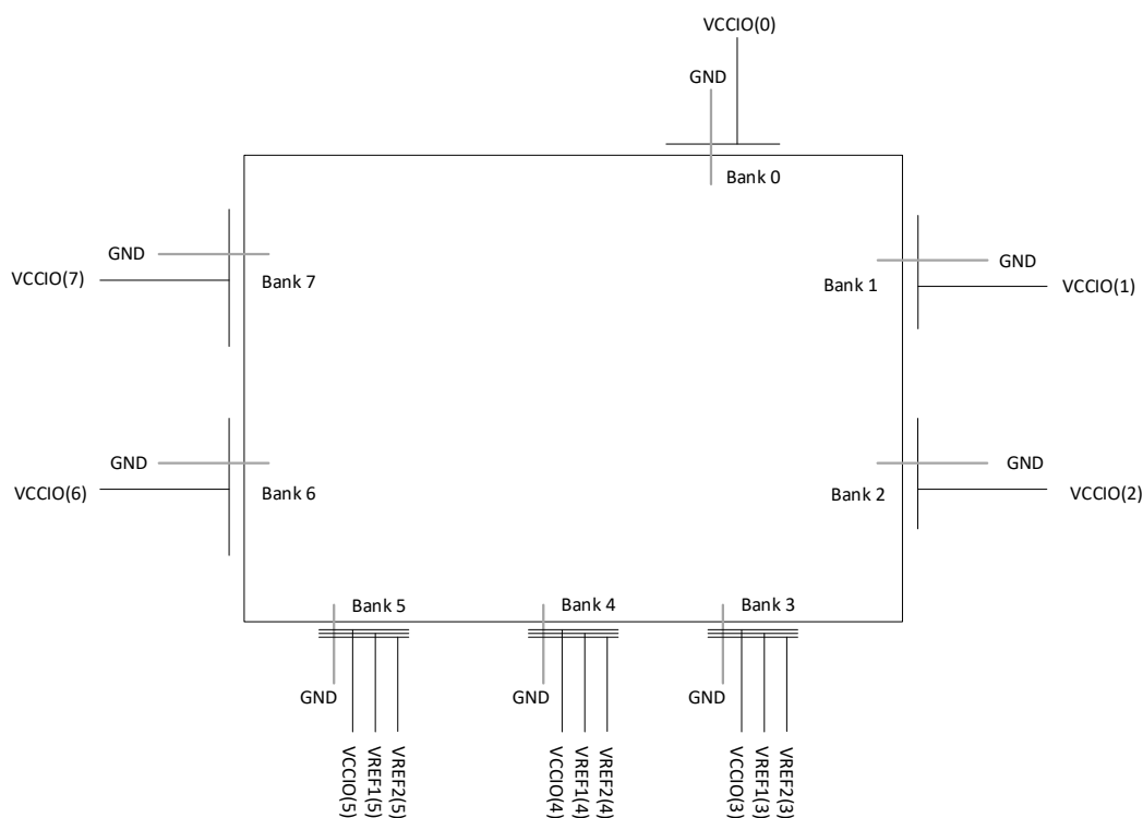
Figure 2.27. sysI/O Banking
