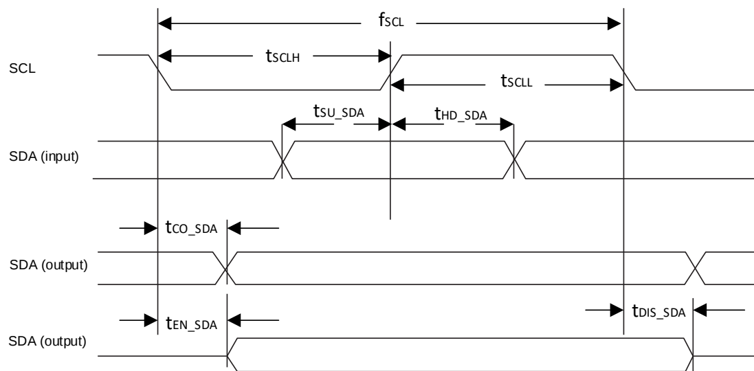
Figure 4.20. I²C/I³C Configuration Timing
