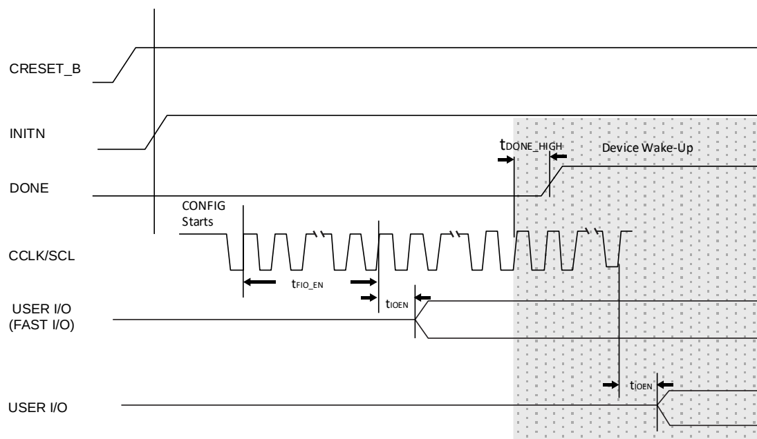
Figure 3.22. Slave SPI/I²C/I³C Wake-Up Timing
