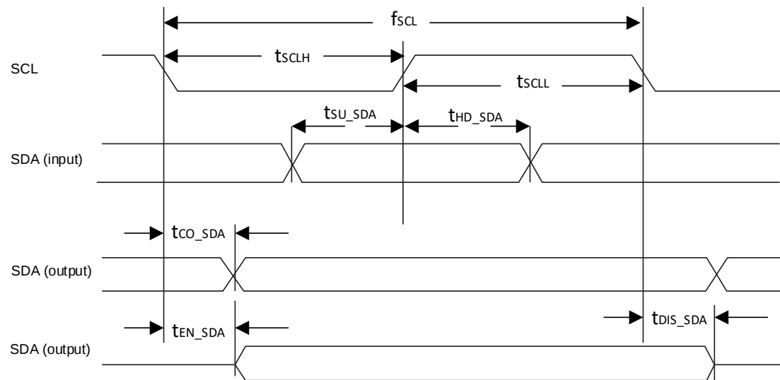
Figure 3.20. I²C/I³C Configuration Timing
