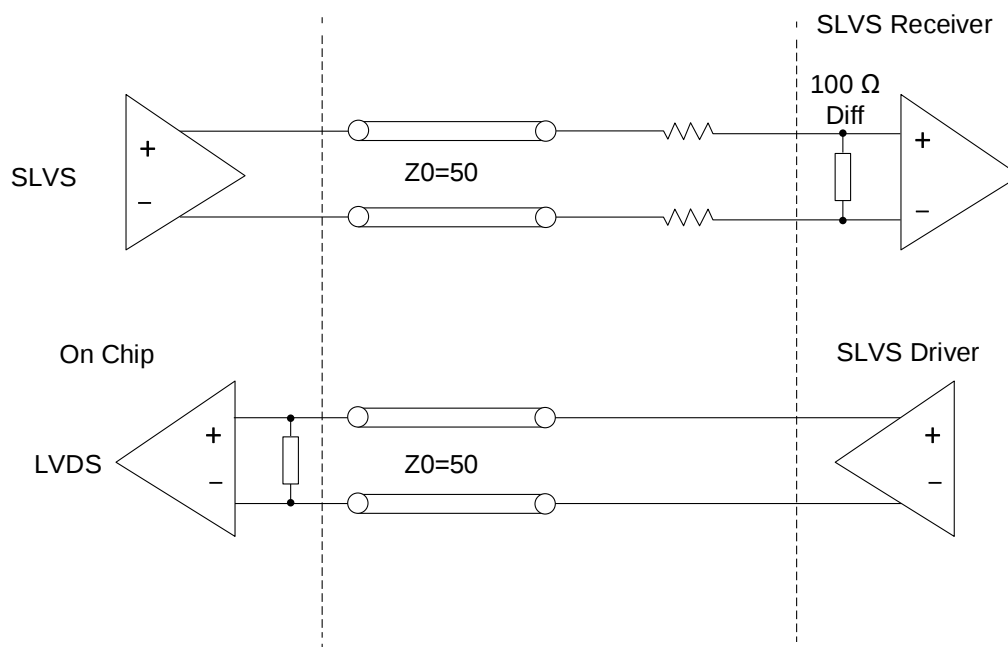
Figure 4.5. SLVS Interface
