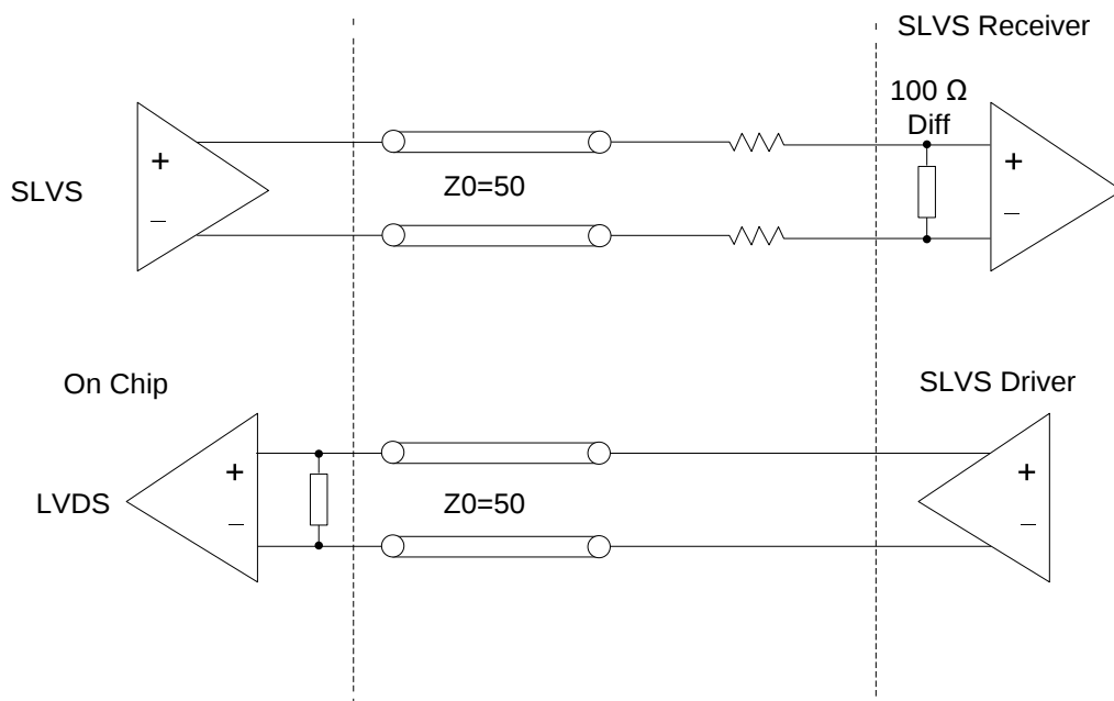
Figure 3.5. SLVS Interface
