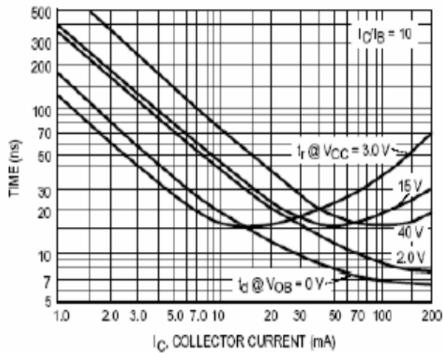
Figure 3 Turn-On Time
