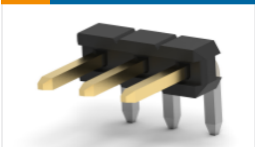
TE Part #2842116-4 4P,2MM,BRK HDR,SRRT,2.8,0.76AU,TB W/CAP
