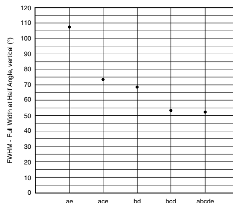
Fig. 3 - Emission Angle vs. Reflector Combination
