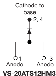
TO-220AB
