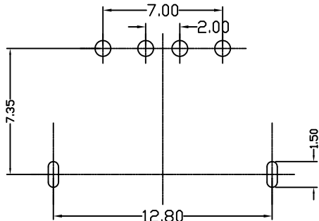
PCB HOLES
