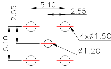
PCB.WELDING DRAWING (TOLERANCE:±0.05)
