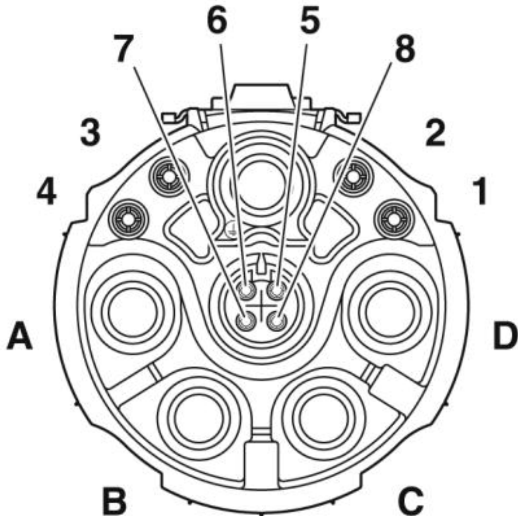
Schematic diagram
